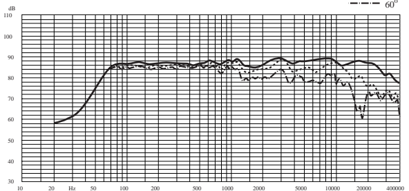
Frequency response (directivity)
