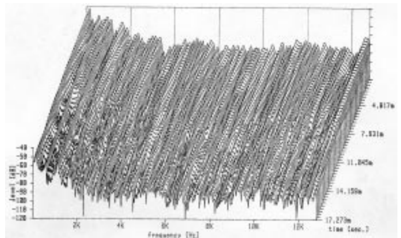
Figure15 without glass wool and HP reflector
